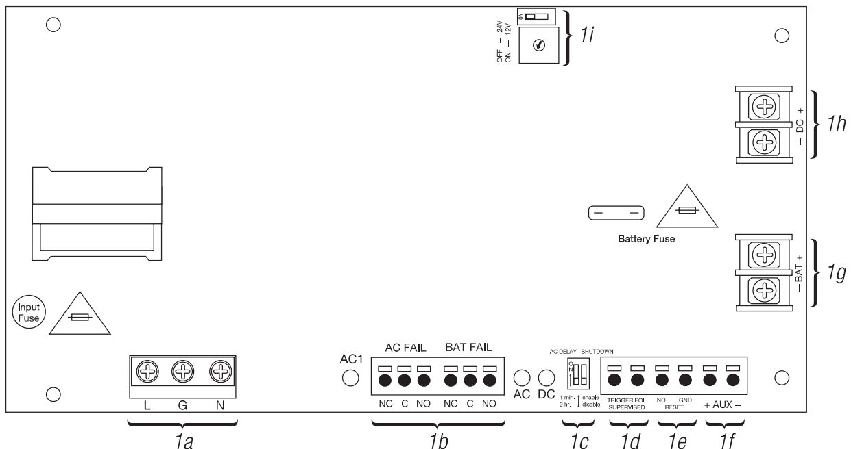
Fig. 1 - eFlowNB Configuration
